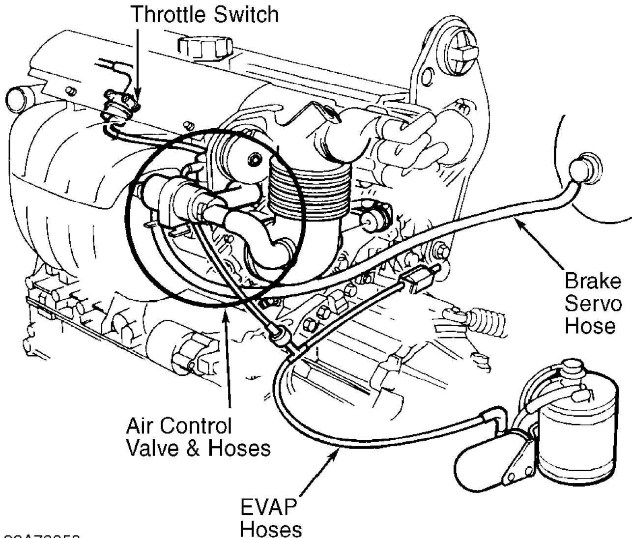
Fig. 1: Identifying Vacuum Hose System Components Courtesy of Volvo Cars of North America.
